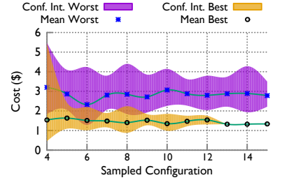
Figure 11: Bayesian opt. process for the best/worst configuration (TeraSort).
