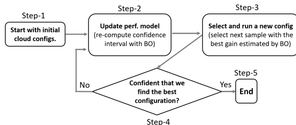
Figure 4: CherryPick workflow
